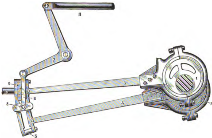
FIG. 238.—Diagram of the Link Motion and Eccentric Gear of a Steam Engine. The parts shown are: (1) backward eccentric; (2) forward eccentric; (3-4) eccentric rods; (5) slotted shifting link; (6) link hanger; (7) reversing arm; (8) link saddle pin; (9) link block; (10) valve stem; (11) reach rod. The position shown in the cut indicates that the backward eccentric is in gear which gives a reverse motion to the engine.
